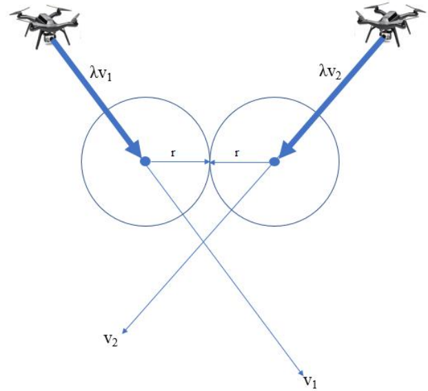
Fig. 6. Collision avoidance between two quadcopters. The original quadcopter trajectories v_1 and v_2 are scaled by the fraction \lambda to produce the modified waypoints.
