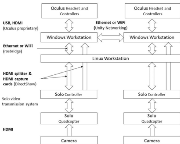
Fig. 1. Hardware and connections
