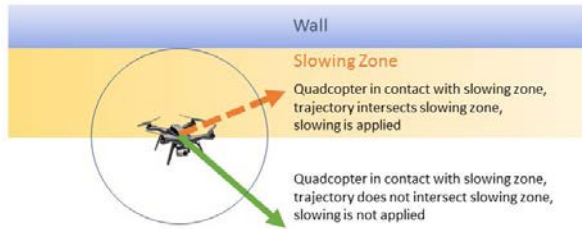
Fig. 7. Waypoint modification to simulate friction with a virtual wall object
